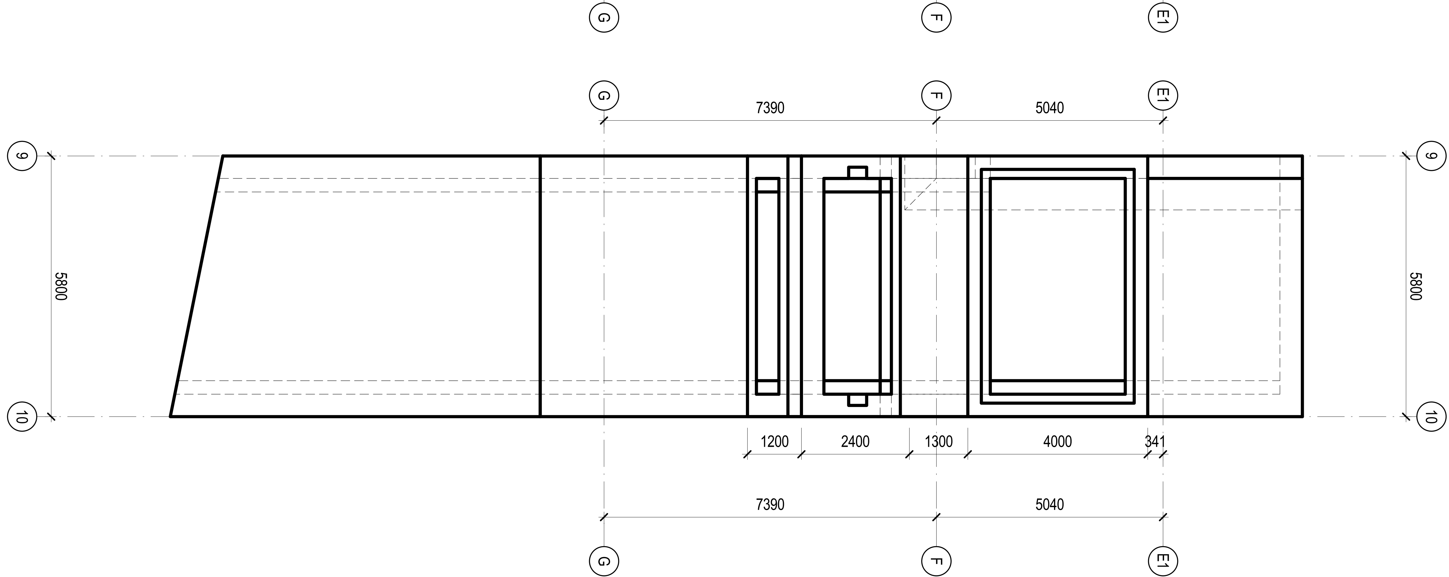
1 1 : 50 PLAN-CELL 9 +2.7
