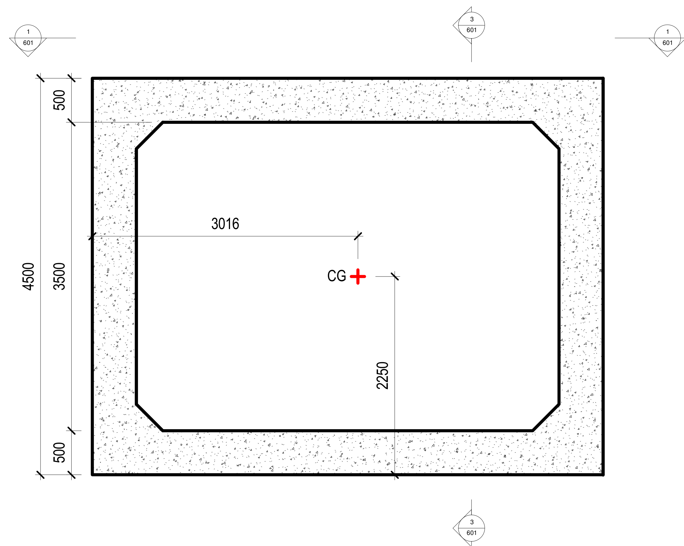
2 DETAIL SECTION A 1 : 25
