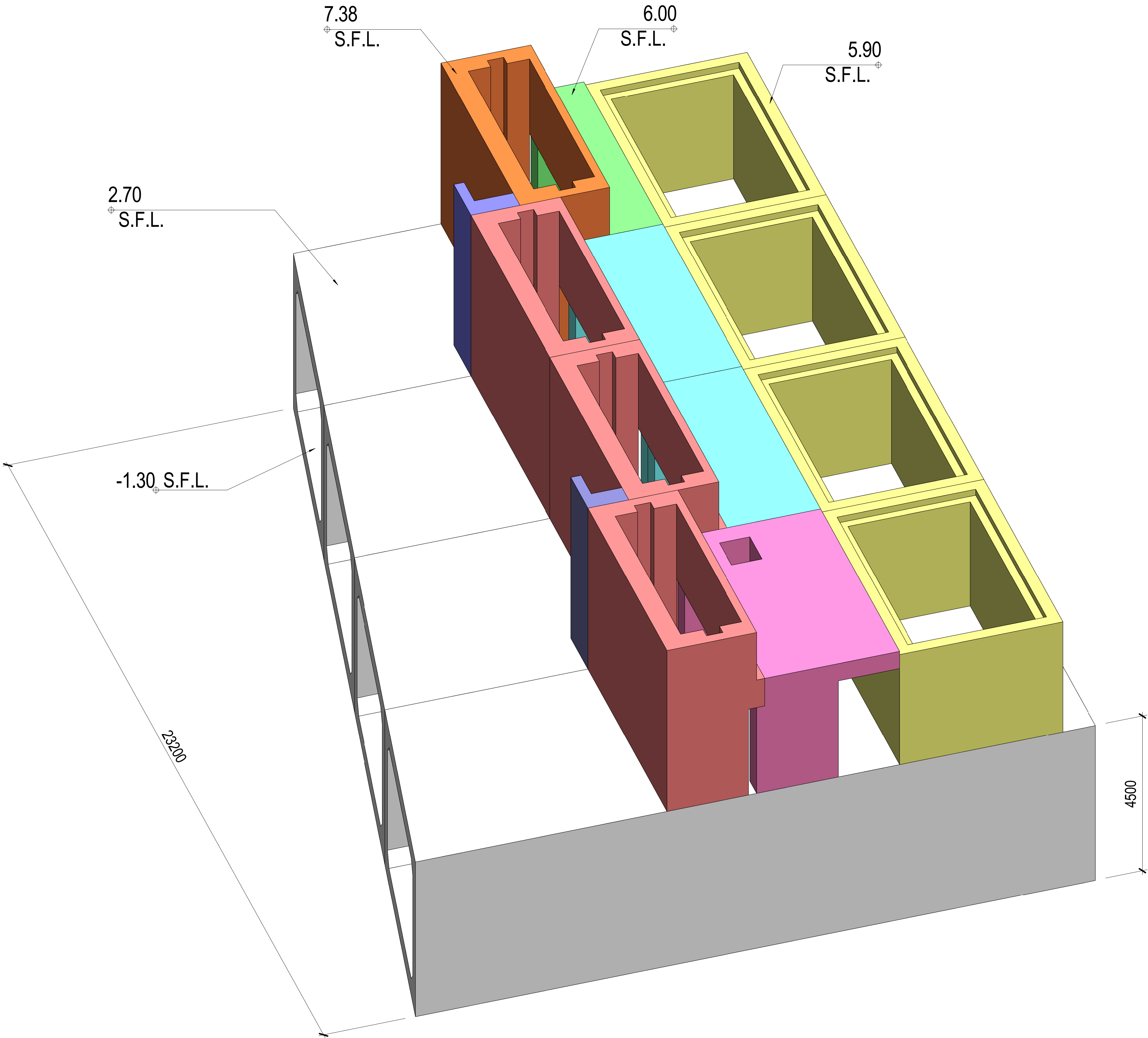
1 ISOMETRIC-CELL 1 TO 4 1:50
