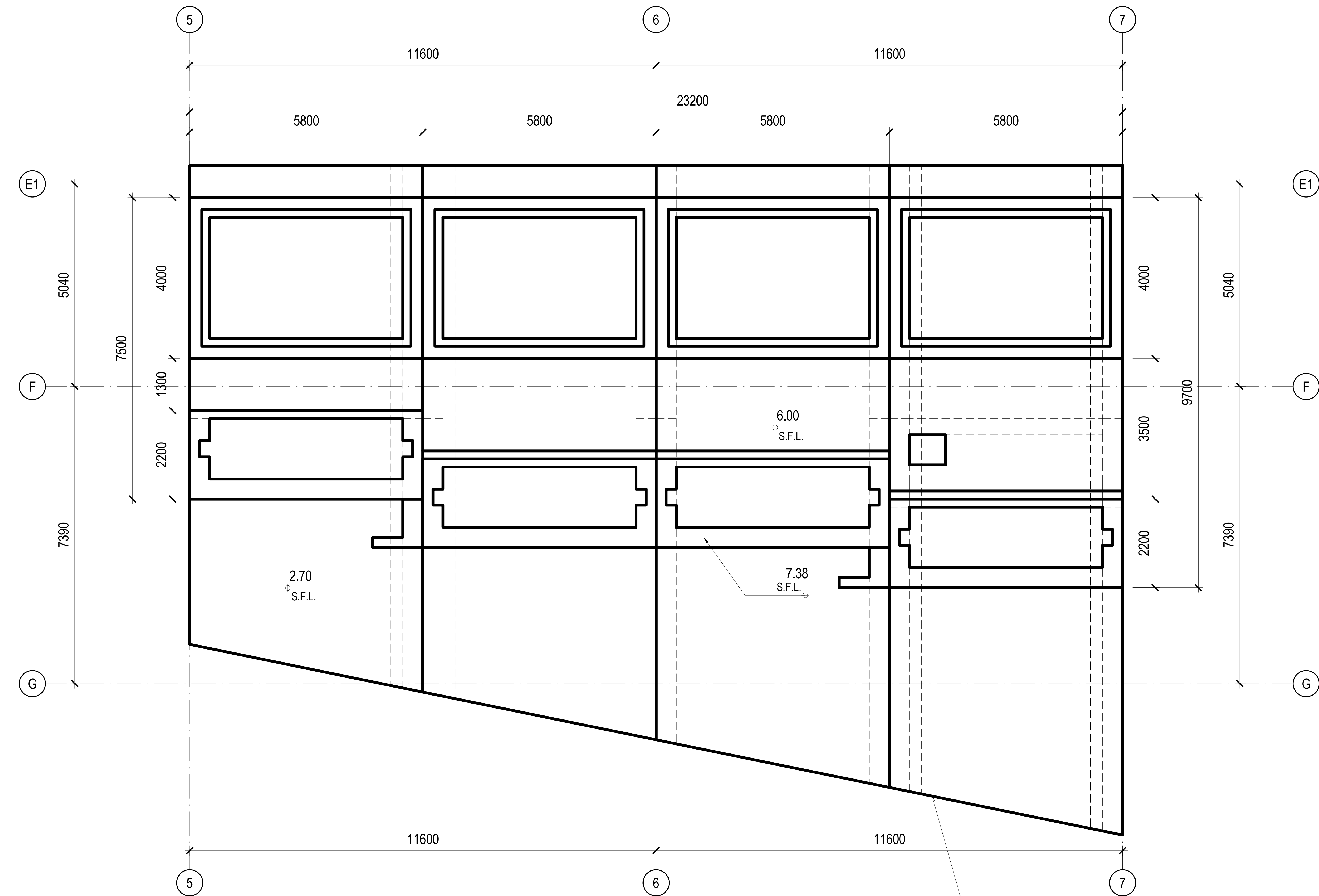
1 PLAN-CELL 1 TO 4 +2.7 1:50
