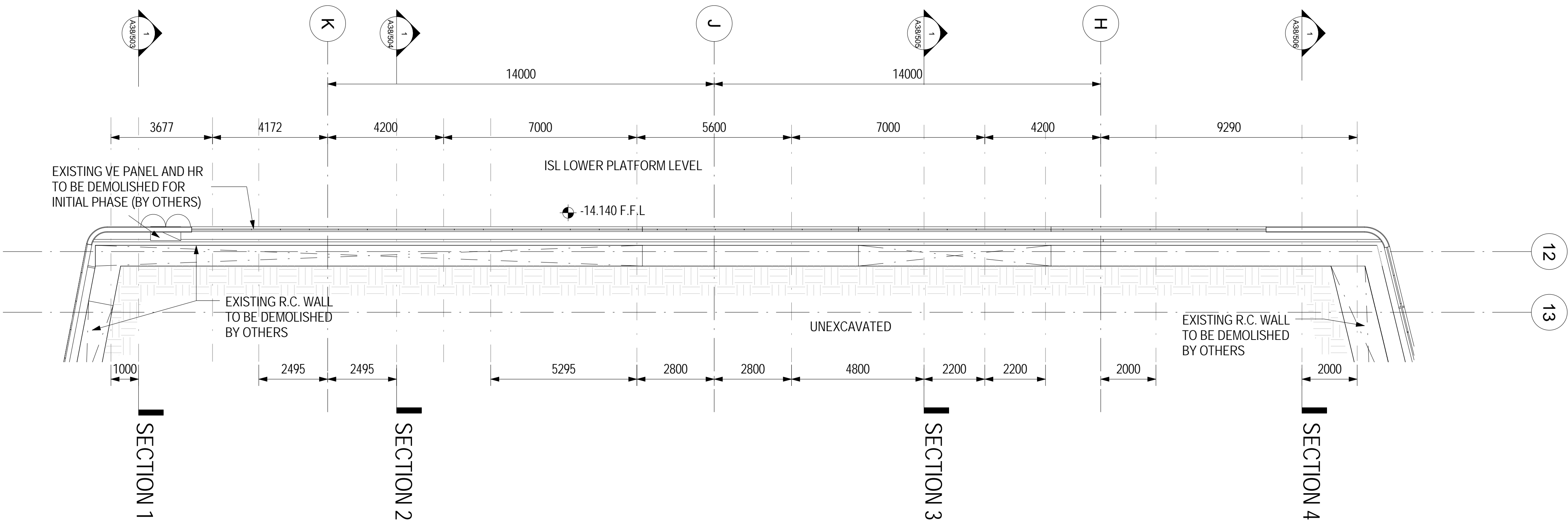
1 EXISTING PHASE - END WALL 1:100
