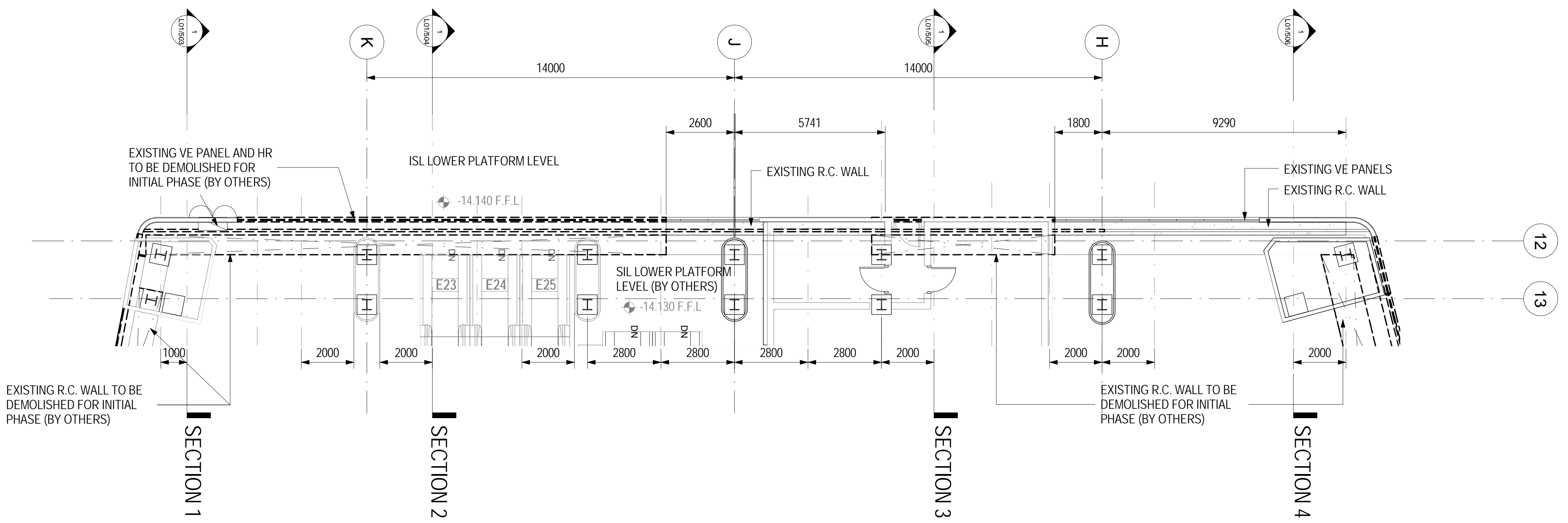
2 INITIAL PHASE - END WALL 1:100
