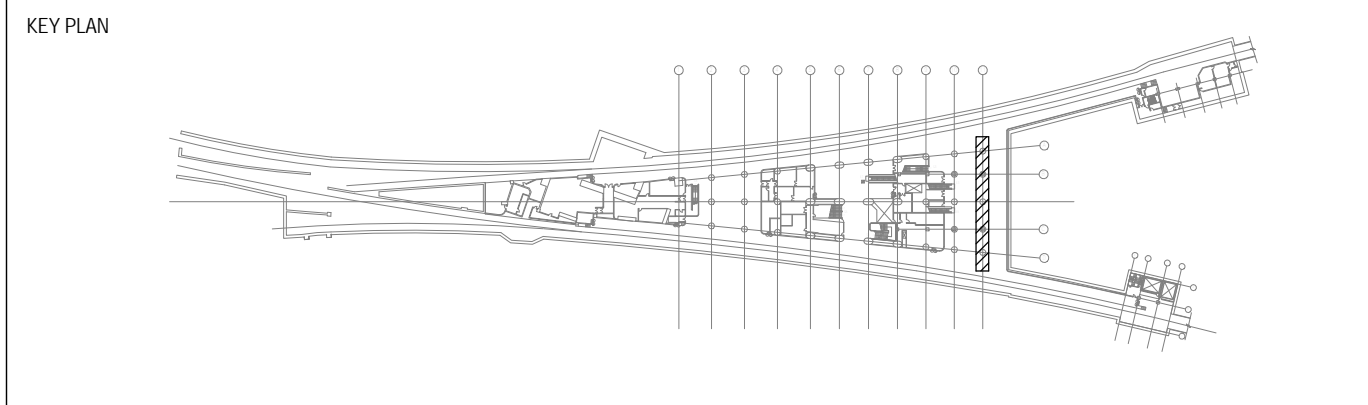
2 INITIAL PHASE - END WALL 1:100
