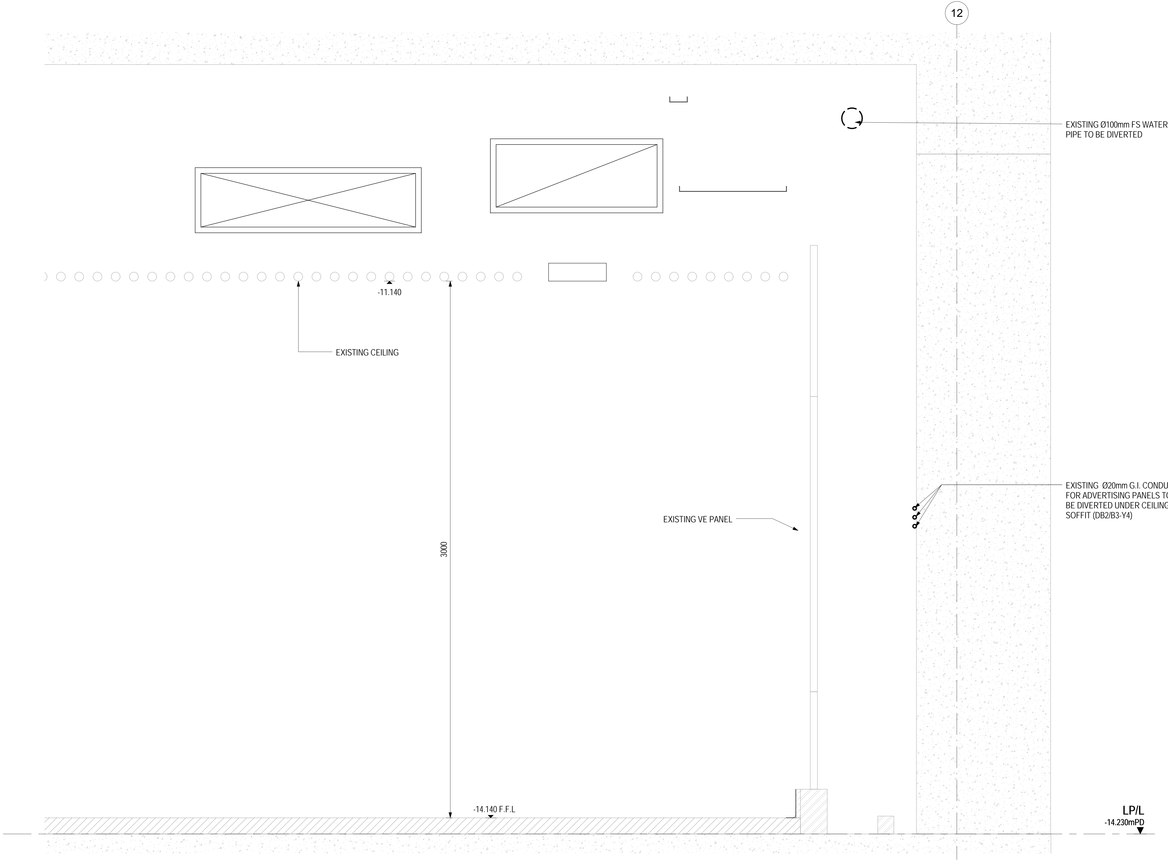
1 EXISTING PHASE_SECTION 4 1 : 10
