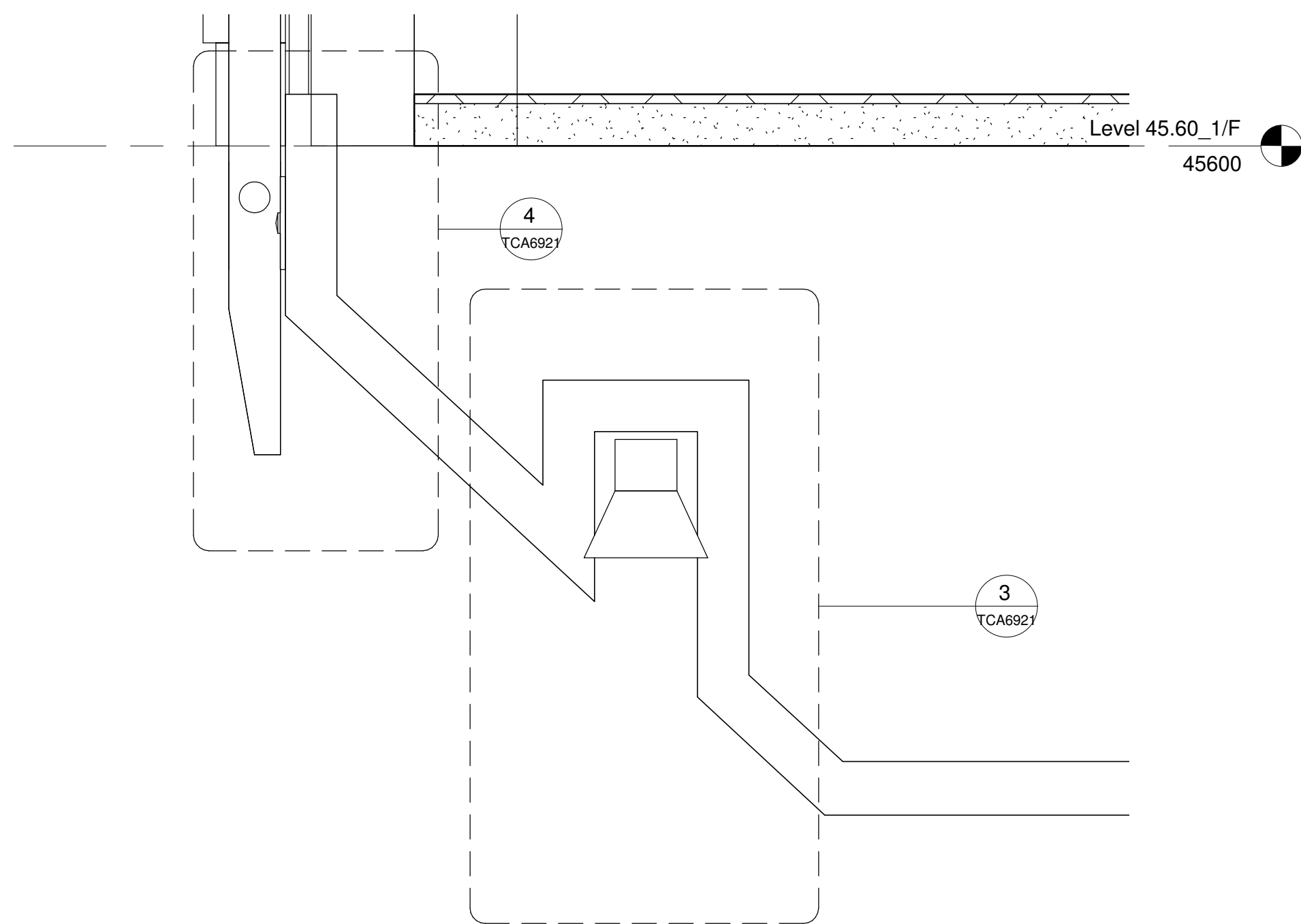
3 Callout of VOID EDGE AT MAIN ENTRANCE 2 1 : 2
