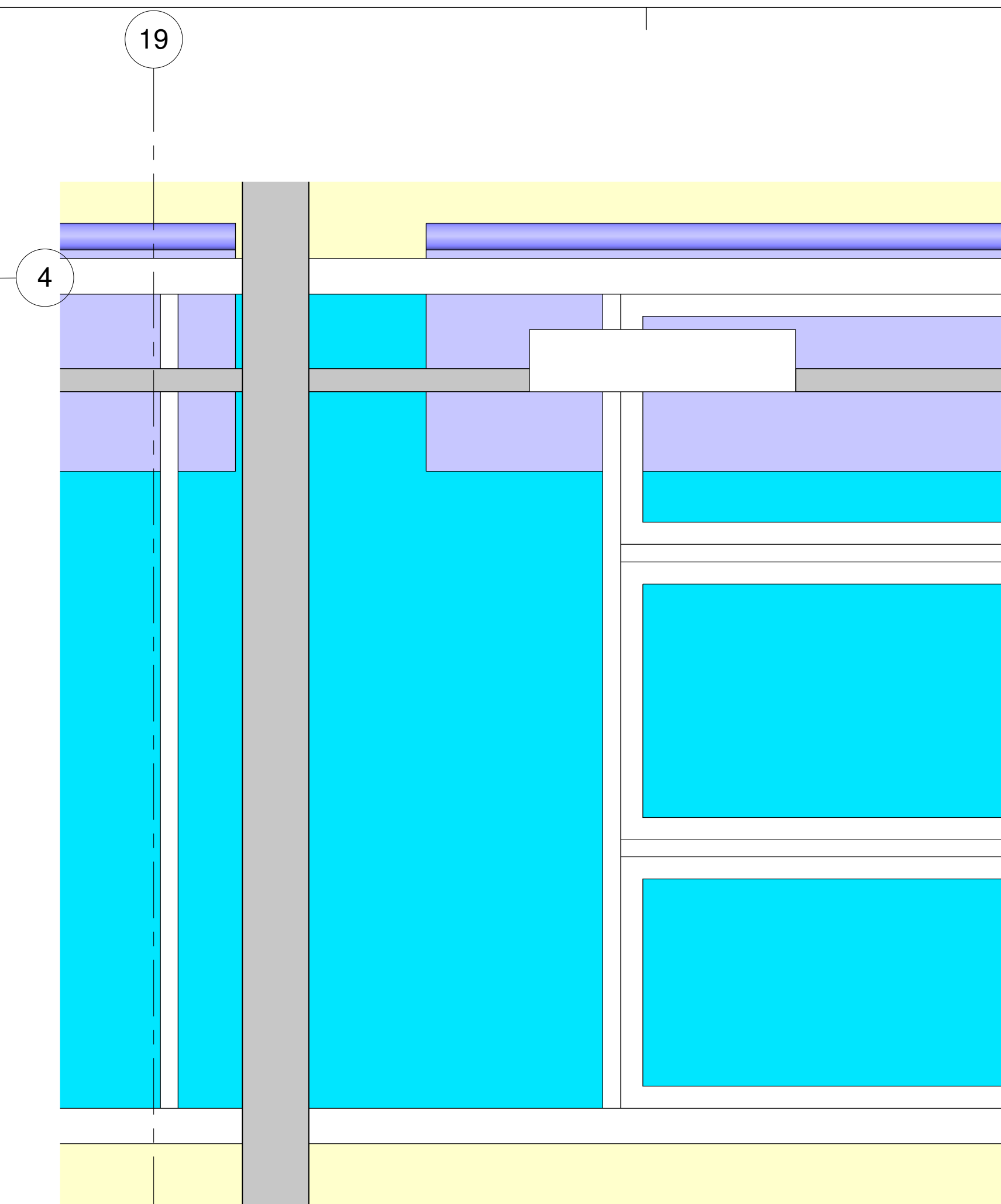
3 Detail of interior condition 2 1 : 10
