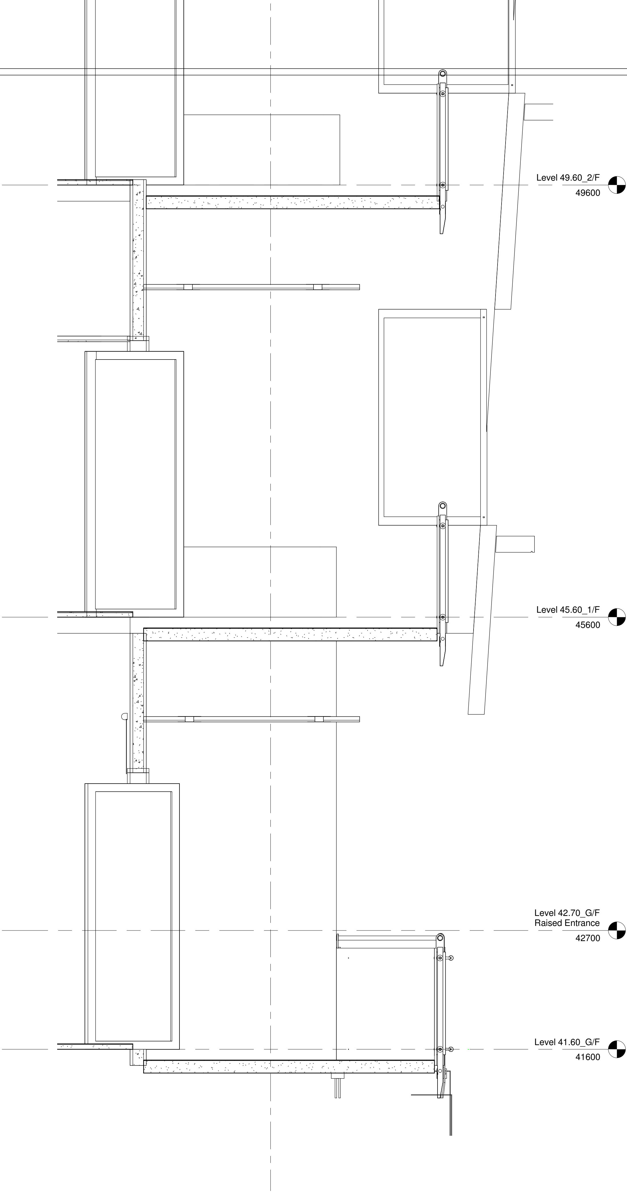
Callout of External Wall Details 06
