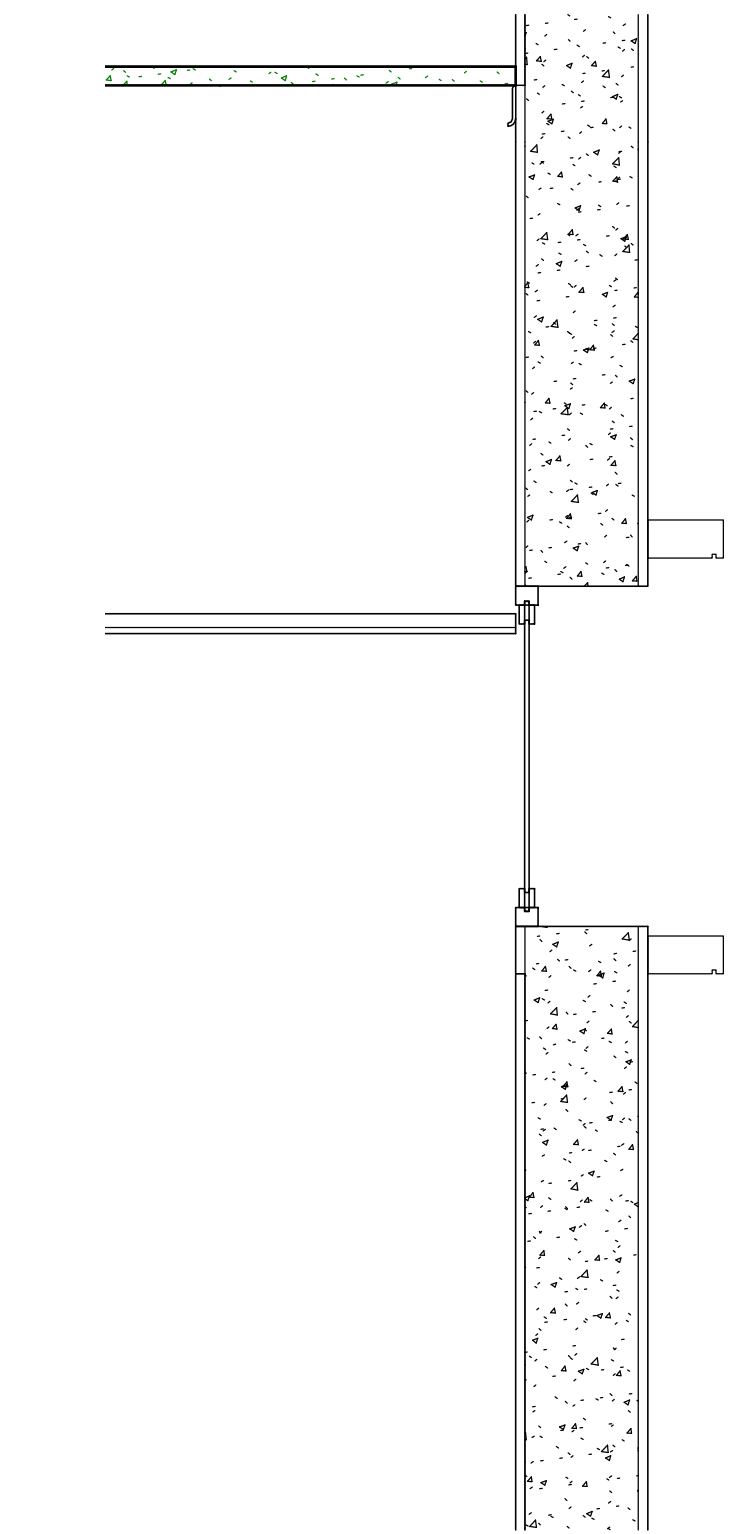
003 Callout of External Wall Details 22 1 : 20
