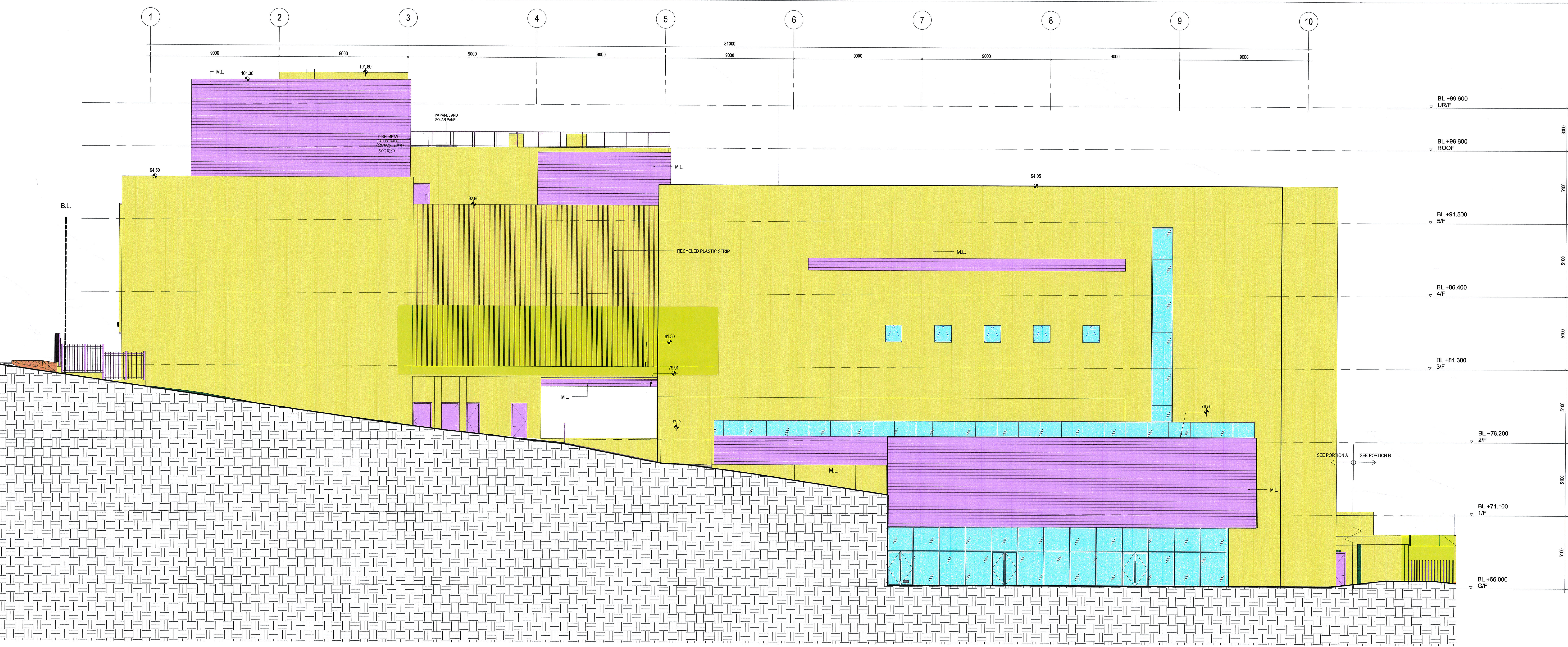
1 ELEVATION (PORTION A) 1:100
