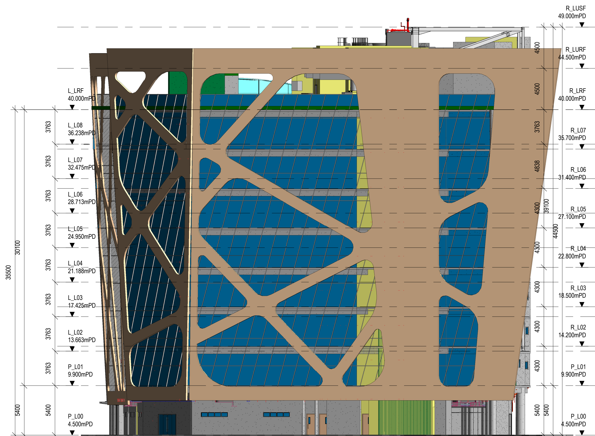
M2 SOUTH ELEVATION 1 : 200
