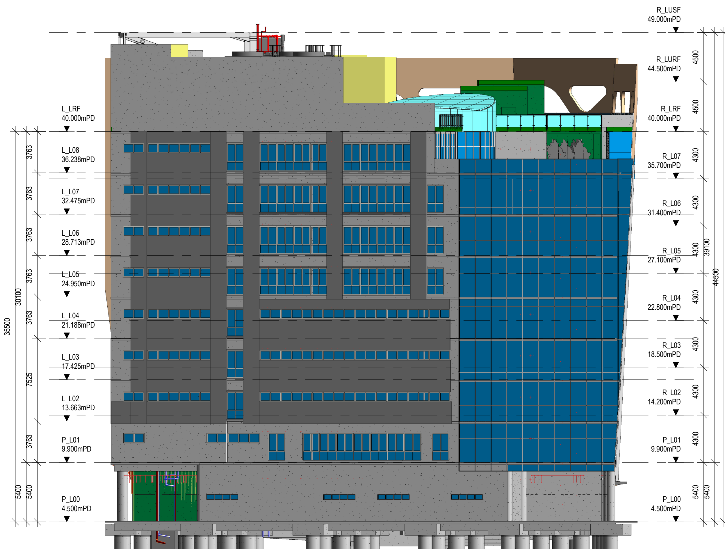
M1 NORTH ELEVATION 1 : 200
