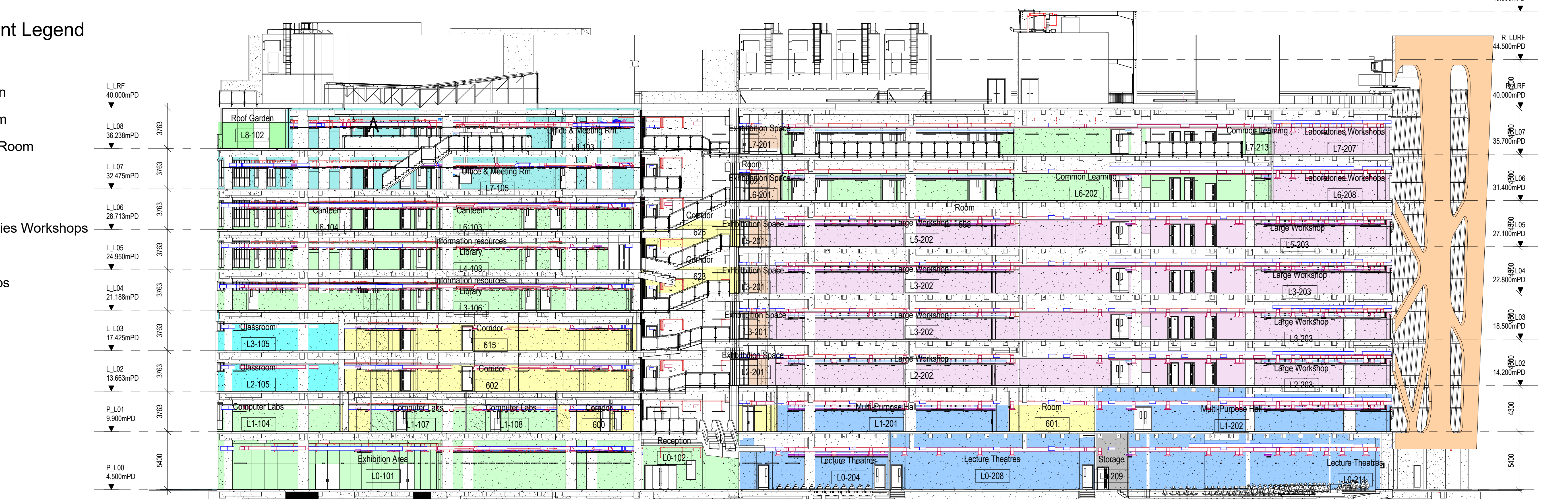
M5 EAST SECTION 1 : 200
