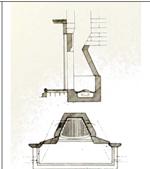
Figure 5: Cross Section and Plan of improved Edwardian fireplace dated 1911. (Source: Richard Russell Laurence)
