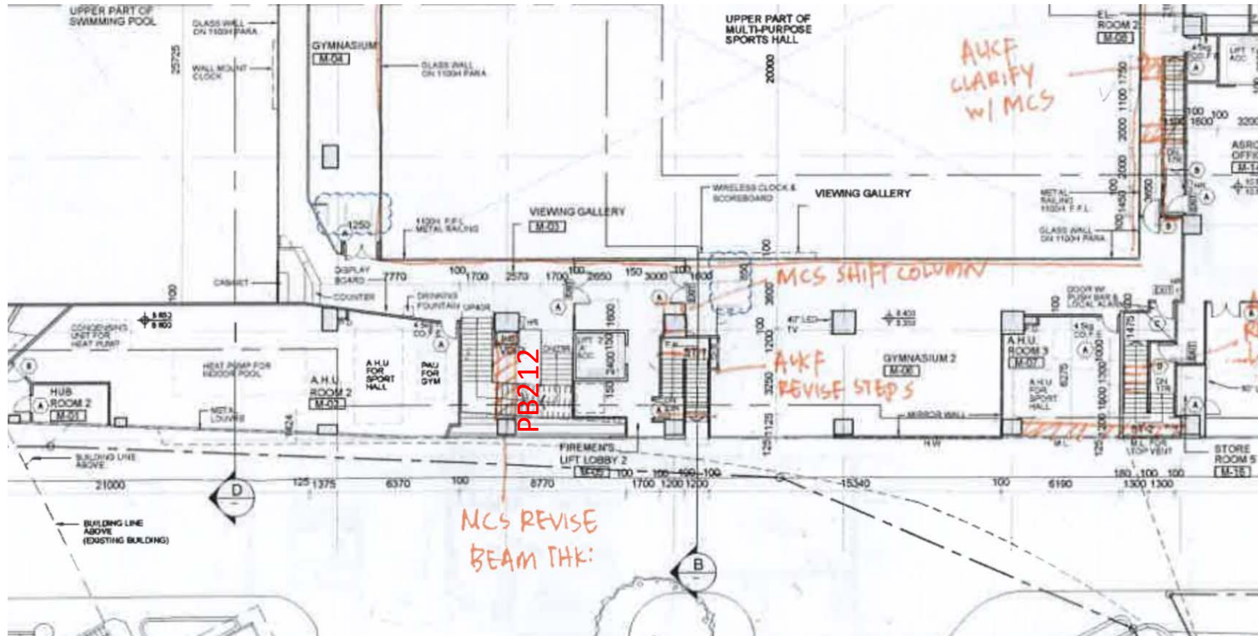
Mezzanine Floor Plan
