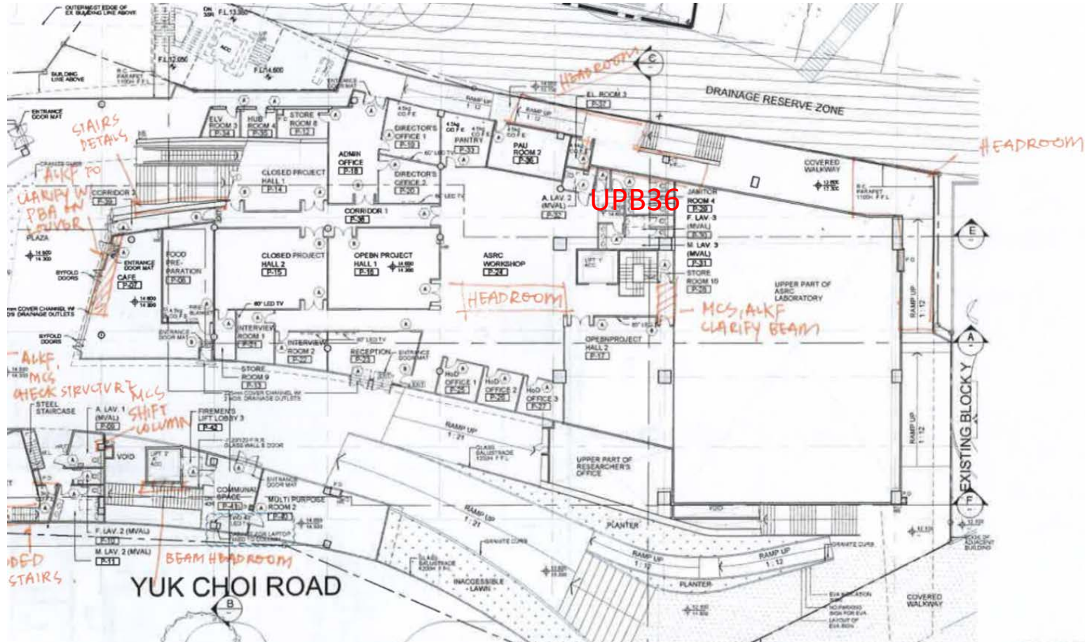
Podium Floor Plan
