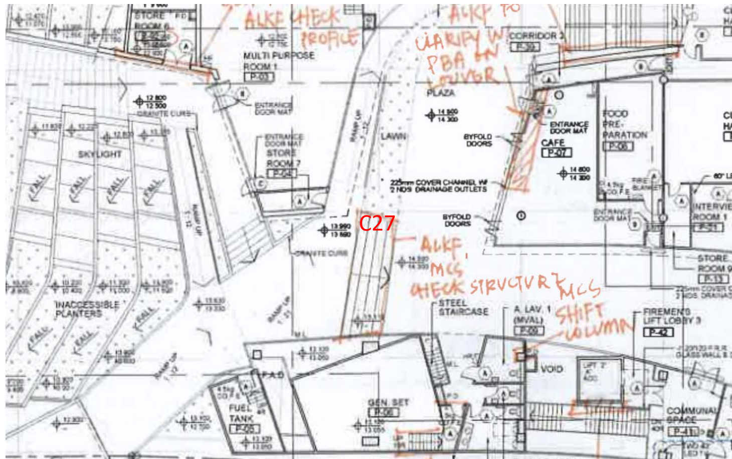
Upper Podium Floor Plan
