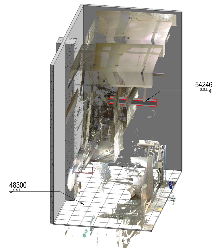
2 3D-Clash 1
